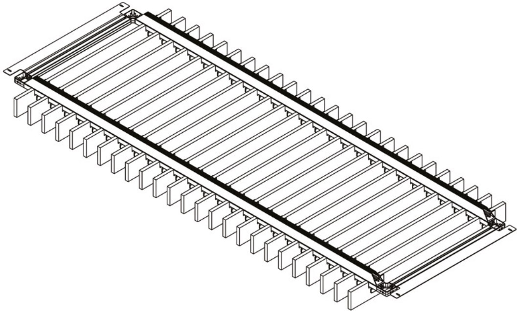
BMGCON-C02 In-between Canopy 2.45m
