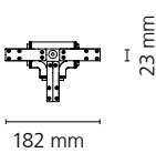
T Joint
