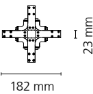
X Joint
